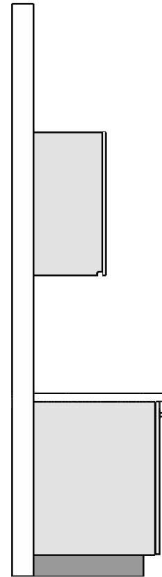
Type 2 Opening - With Wall Gola Profile EVA CALYPSO *Suitable for exposed sidepanel
