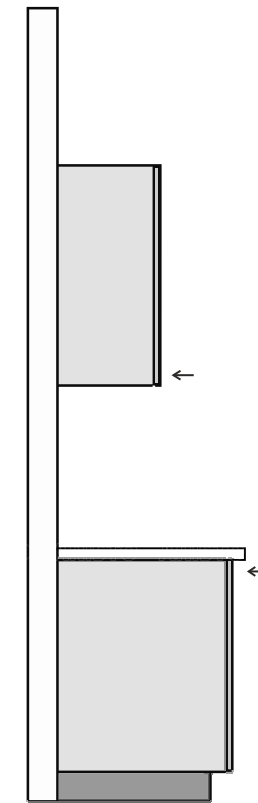
TYPE4 Opening - With Servo drive/ Push Open
